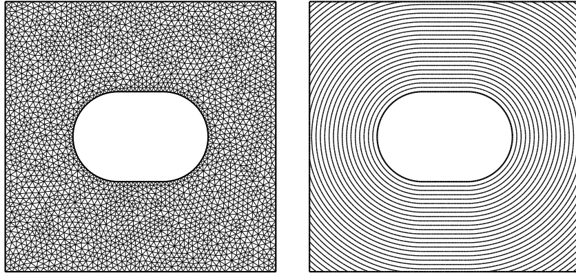
Figure 12: Smooth Eikonal Solns: Coarsest Mesh (left) and Solution (right).
