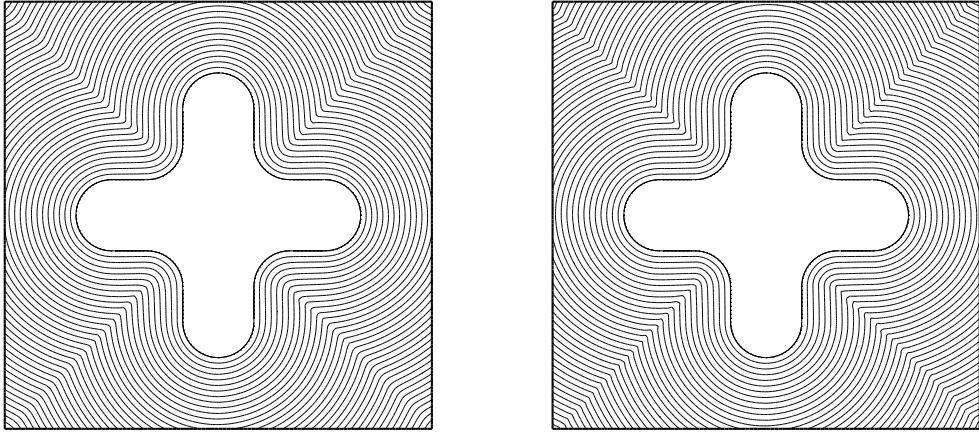
Figure 7: Level set solution obtained using monotone scheme with virtual edge flipping (left) and positive coefficient scheme (right).
