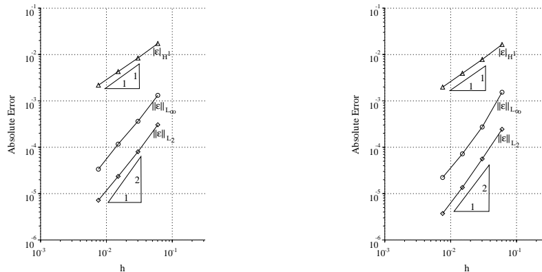
Figure 13: Smooth Eikonal Solns: Absolute solution error. Positive coefficient scheme (left), explicit Petrov-Galerkin (right).
