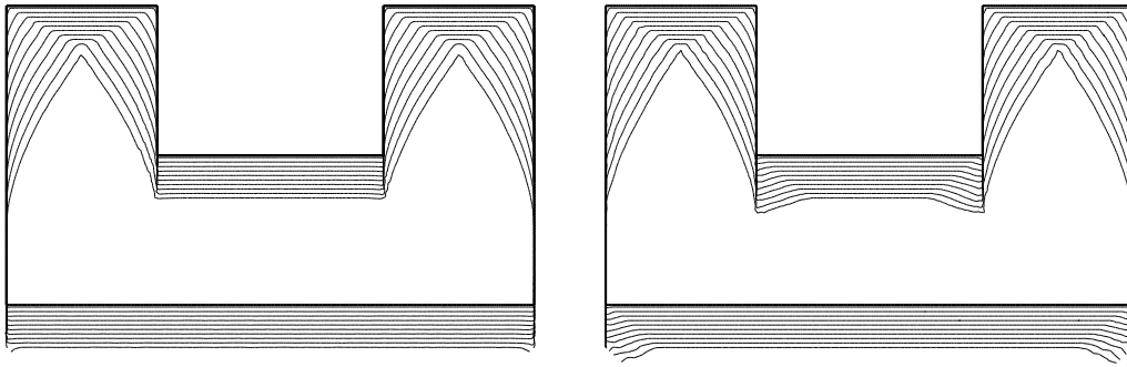
Fig. 25c. Exp. Petrov-Galerkin + D.C. Fig. 25d. Imp. Petrov-Galerkin + D.C.
