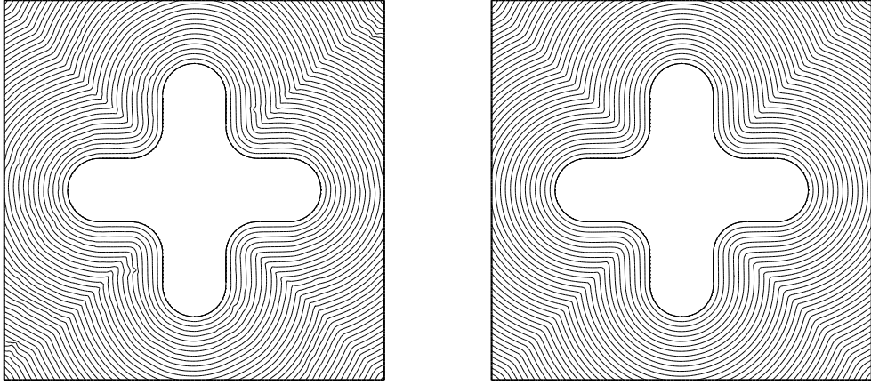
Figure 5: Level set solutions obtained without (left) and with (right) virtual edge flipping.
