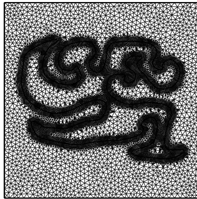
Initial Adapted Mesh
