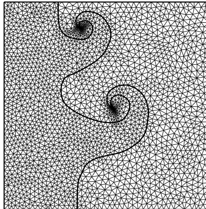
Fig. 18c. Interface Conforming Adaptation.
