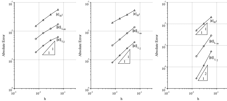
Figure 11: Smooth Level Set Solns: Absolute crossing time solution error. Positive coefficient scheme (left), explicit Petrov-Galerkin (middle), and implicit Petrov-Galerkin (right).
