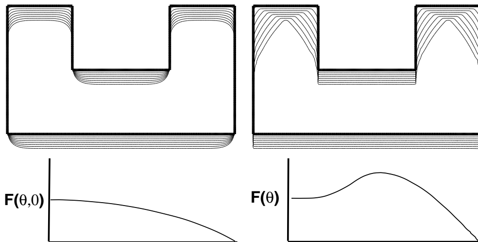
Fig. 24c. F(\theta, \kappa) = \cos \theta - .1\kappa .
