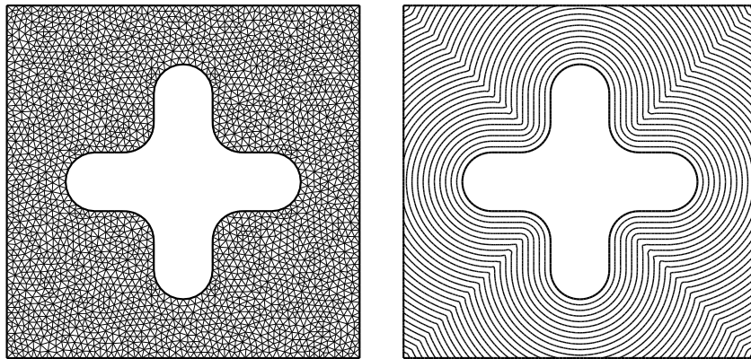
Figure 16: Non-Smooth Eikonal Solns.: Coarsest Mesh (left) and Solution (right).
