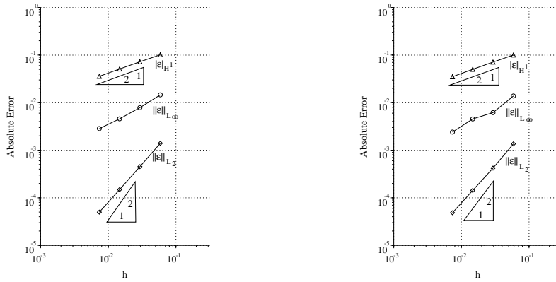
Figure 17: Non-Smooth Eikonal Solns.: Absolute solution error. Positive coefficient scheme (left), Petrov-Galerkin (right).
