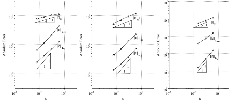
Figure 15: Non-Smooth Level Set Solns: Absolute crossing time solution error. Positive coefficient scheme (left), explicit Petrov-Galerkin (middle), and implicit Petrov-Galerkin (right).
