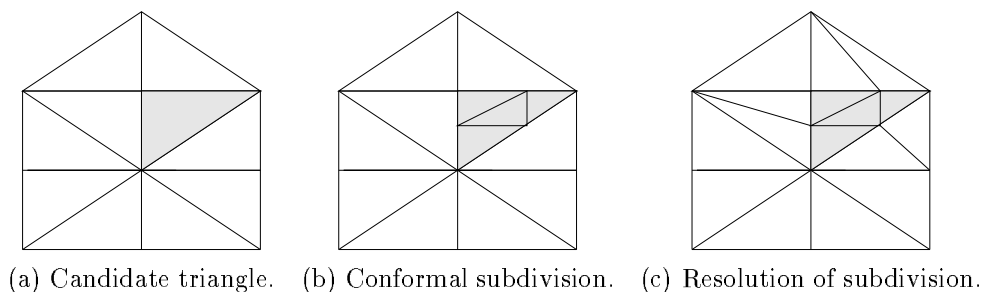
Figure 19: Conformal refinement steps for a 2D triangle.
