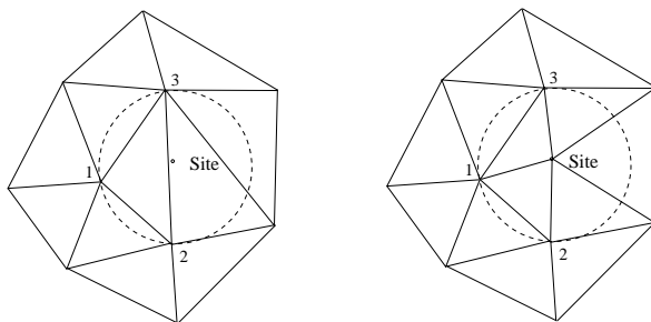
Figure 20: Steiner refinement: Site insertion at circumcenter location (left) and edge reconfiguration (right).
