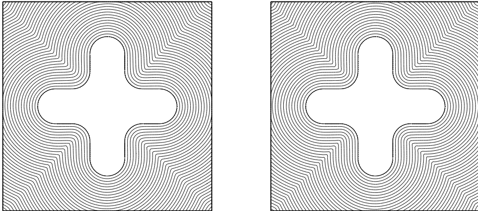
Figure 8: Level set solution obtained using monotone scheme with virtual edge flipping (left) and Petrov-Galerkin scheme (right).
