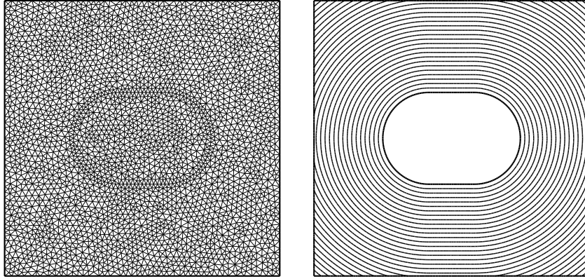
Figure 10: Smooth Level Set Solns: Coarsest Mesh (left) and Crossing Time Solution (right).
