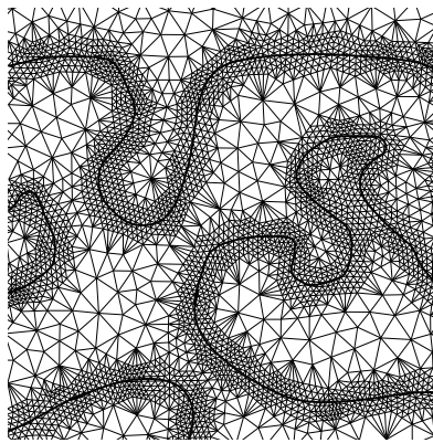
Fig. 18a. Interface proximity adaptation. Fig. 18b. Curvature adaptation.
