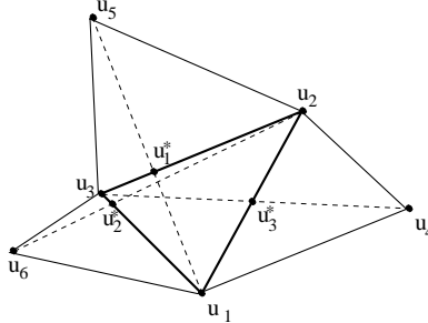
Figure 4: Virtual edge flipping strategy. Given the triangle T(v_1, v_2, v_3) with vertex solution values u_1 , u_2 , and u_3 , additional solution values u_1^* , u_2^* , u_3^* and positions are computed based on (virtual) diagonal flipped edges e(v_3, v_4) , e(v_1, v_5) , e(v_2, v_6) .
