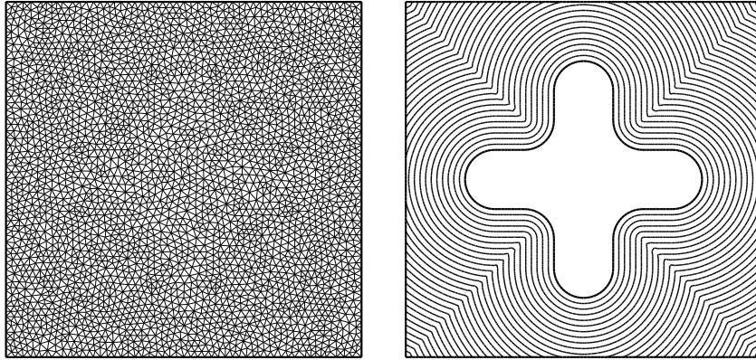
Figure 14: Non-Smooth Level Set Solns.: Coarsest Mesh (left) and Crossing Time Solution (right).
