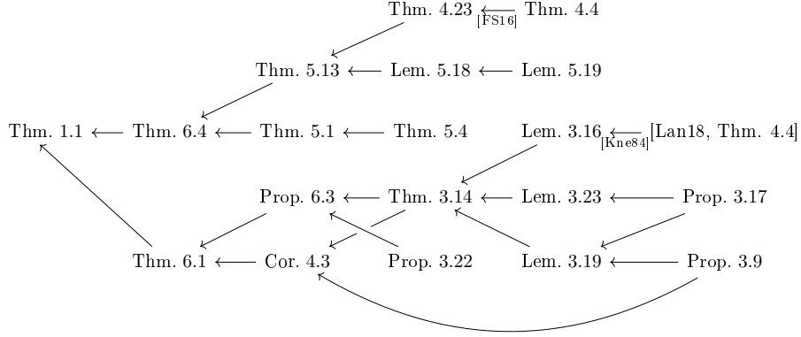
FIGURE 1. A schematic diagram depicting the structure of the proof of Theorem 1.1.
