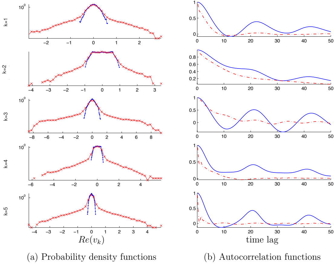
Figure 6: Results produced by ARMAX, i.e., using only linear terms in the ansatz for z^n . In (a), we compare the probability density functions of different modes produced by ARMAX (red 'x's) to that of the full model (blue dots). In (b), we compare the autocorrelation functions (solid line for full model, dashed line for ARMAX). Compare to Figures 2(b) and 3(b).
