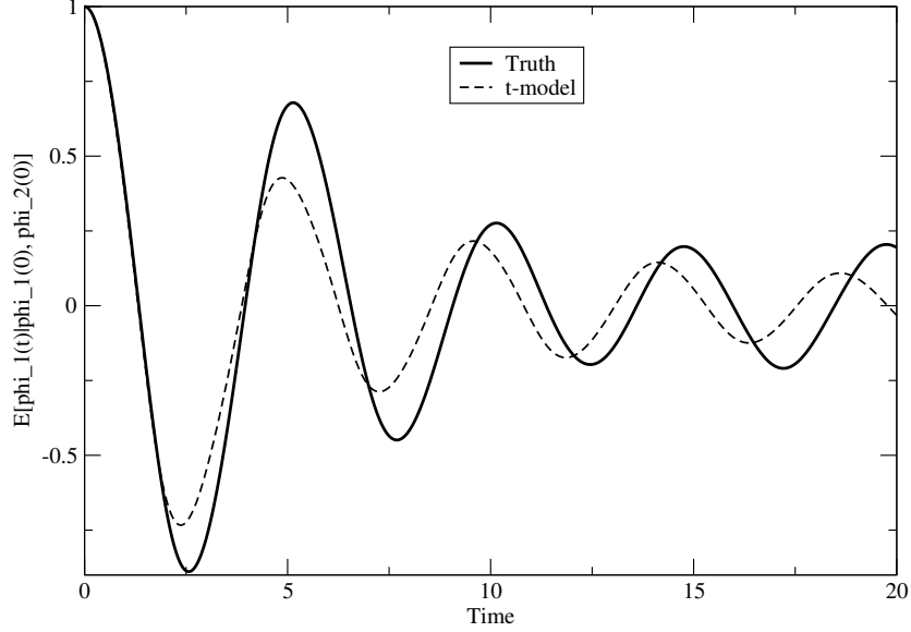
Figure 2: Comparison of the evolution of E[\phi_1(t)|\phi_1(0), \phi_2(0)] (truth) with the prediction by the t-model; for comments, see the text.
