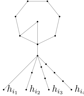
FIGURE 1. We call this configuration an m -spider, where m is the size of the top loop ( m = 7 in this case). The edges represent the pairs of elements that satisfy E . Let \ell_m be the number of nodes in the spider ( \ell_m = 13 in this case).
