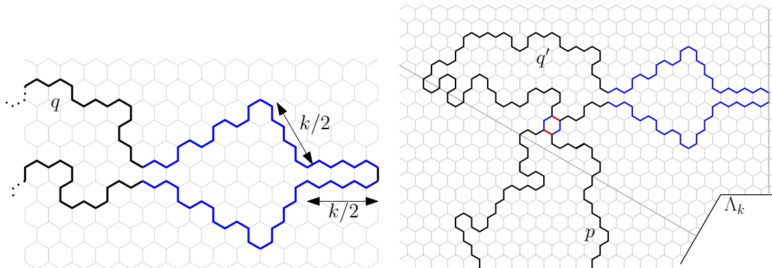
FIGURE 11. Left: Construct q' by joining to the rightmost edge of q the blue polygon shaped as an arrow. Right: The polygon q' is manoeuvred along \ell into a position whereby it may be joined to p via the indicated hexagon. In this instance, the join occurs by the removal of the two red edges and the addition of the four blue ones.
