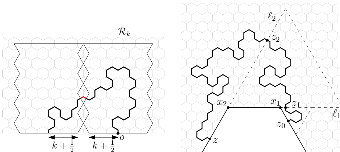
FIGURE 10. Left: The domain \mathcal{R}_k and a translate of it. Two walks contributing to G_{\mathcal{R}_k}(o, z) for some z \in \text{Left}'_k (one is reflected and translated) may be used to create an arc of between o and (-2k - \frac{1}{2}, 0) . The red edges are added in the concatenation Right: To connect z_0 to z we use (7.6) to arrive to some point z_i on the same line as z , then use (7.7) to connect z_i to z .
