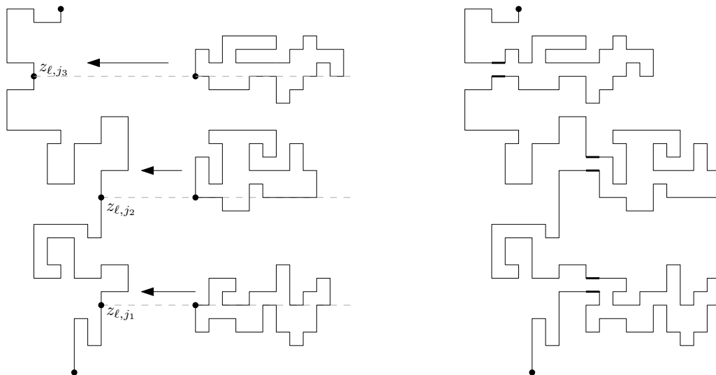
FIGURE 5. A toy depiction of the Madras join of a branch \phi^{(\ell)} and three polygons p_{(\ell, j_1)} , p_{(\ell, j_2)} and p_{(\ell, j_3)} at respective heights j_1 , j_2 and j_3 . The edges introduced in surgery have been represented merely by two thick edges in each case.
