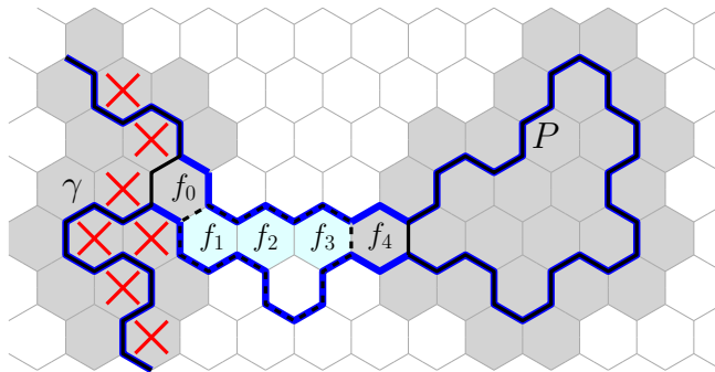
FIGURE 12. The join M(\gamma, P) is emboldened. The grey faces are part of F(\gamma) and F(P) ; the bad faces of \gamma are marked. The choice of f_0 and f_4 may be such that both are good. The polygon Q is dotted.
