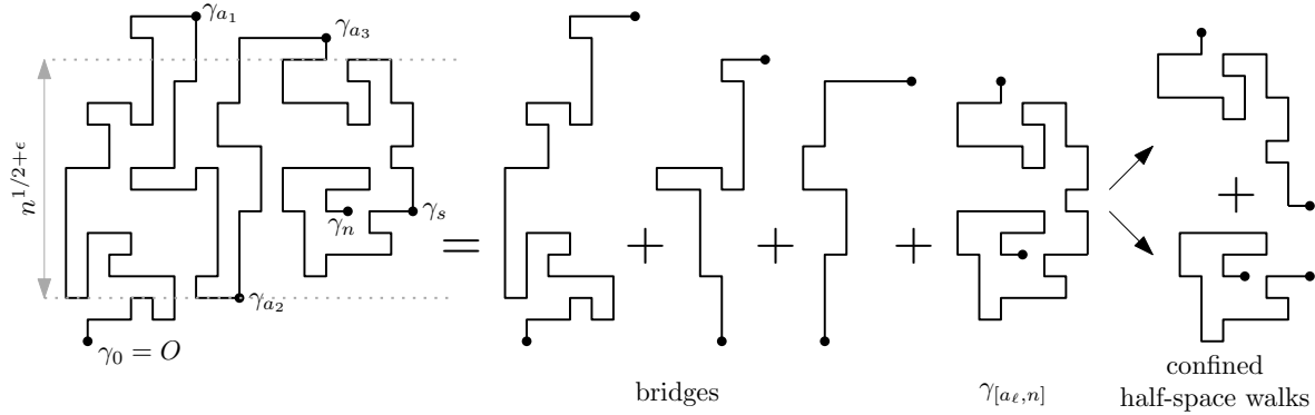
FIGURE 4. A half-space walk is decomposed into three bridges of height larger than n^{1/2+\epsilon} and a final piece of height smaller than n^{1/2+\epsilon} . The latter is decomposed into two (rotated) confined half-space walks.
