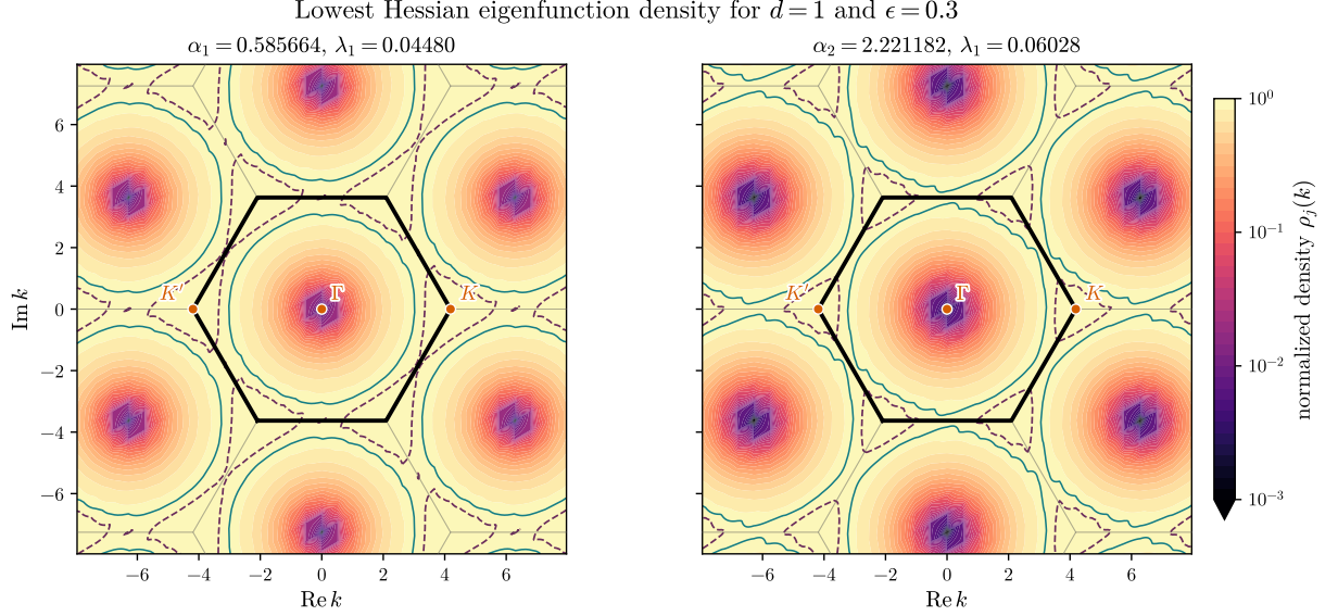
FIGURE 1. Numerically computed lowest eigenfunctions, \psi_1 (with the eigenvalues \lambda_1 determining the constants in (1.2)) for the first two magic angles of [TKV19]: the plot shows the log of the normalised density, \rho_j(k) := |\psi_1(k)|^2 / \max_q |\psi_1(q)|^2 , for \alpha_j , j = 1, 2 . The parameters in (1.1) are d = 1 and \epsilon = 0.3 . The vanishing at \Gamma = 0 follows from basic symmetries. This figure and Figure 2 were produced, on request, by ChatGPT 5.6.
