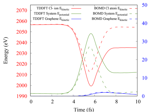
Figure 5. BOMD and RT-TDDFT energy transfer with time; the projectile speed is 2.0 Bohr/fs.
