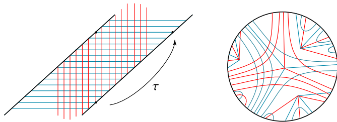
FIGURE 4 The orbit space of a skew flow (left) and a schematic of that of a pseudo-Anosov flow (right). Nonseparated stable and unstable leaves “meeting at infinity” define a shift \tau commuting with the action of \pi_1(M) on the skew picture.
