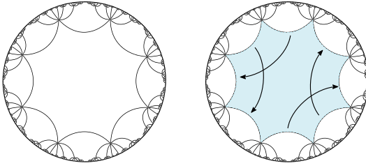
FIGURE 1 A regular tiling of the hyperbolic plane by octagons with geodesic sides. The symmetries of this tiling is a hyperbolic group with boundary S^1 . Identifying sides of the octagonal domain by translations indicated on the figure gives a genus 2 surface with hyperbolic structure.
