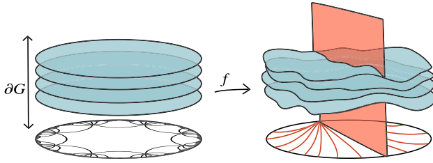
FIGURE 3 An equivariant map locally close to the identity on \tilde{M} \times \partial G captures a perturbation of the action of G = \pi_1(M) on \partial G . The images of horizontal leaves \tilde{M} \times \{x\} intersect the leaves of the stable foliation of geodesic flow (in red) along quasigeodesics allowing us to use large-scale metric stability to prove dynamical stability. For general groups, one needs a more complicated space and a substitute for the stable foliation.
