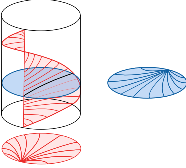
FIGURE 2 UT(\mathbb{H}^2) is trivialized as \mathbb{H}^2 \times S^1 , where the point on S^1 (height) is given by the endpoint at infinity of a geodesic ray with given tangent vector. Leaves of the weak-stable foliation are horizontal, weak-unstable leaves intersect them transversely along geodesics.
