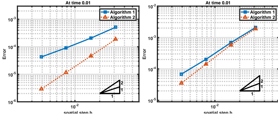
FIGURE 3. Convergence plot, Left : Structured mesh, Right : Unstructured mesh.
