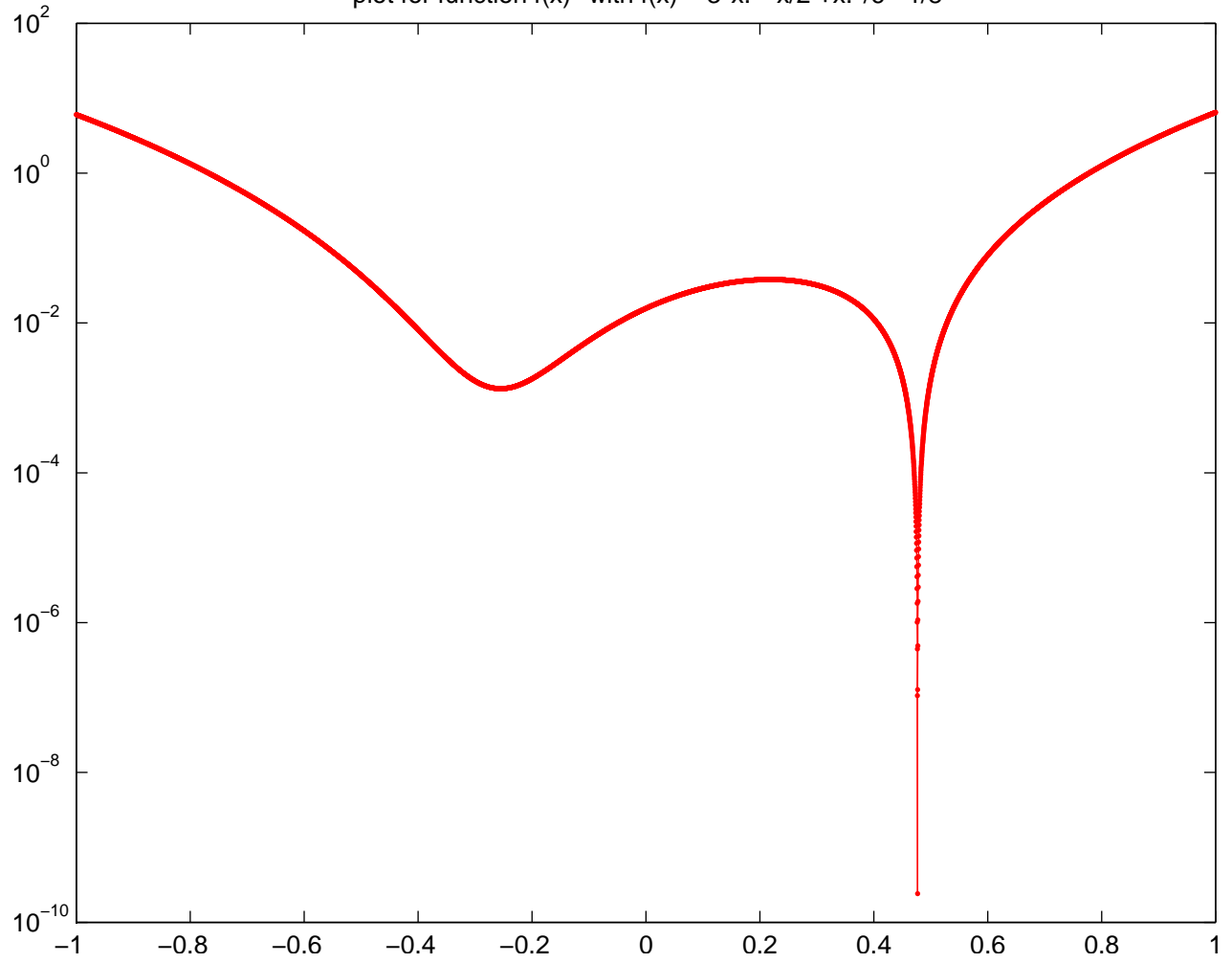
plot for function f(x)^2 with f(x) = 3 \cdot x^3 - x/2 + x^2/6 - 1/8
