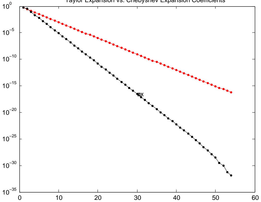
Taylor Expansion vs. Chebyshev Expansion Coefficients
