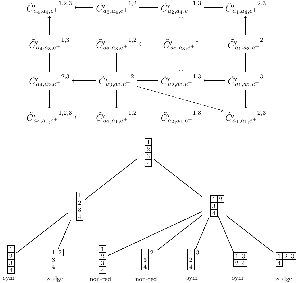
FIGURE 1. The W -graph on \mathcal{H} \otimes_{J'_{n-1}} \mathcal{H} \otimes_{J'_{n-1}} e^+ and the graph G of §3.4. The vertices of the tree G are marked by local labels. Each cell in the W -graph corresponds to the path from a leaf to the root that is its local sequence.
