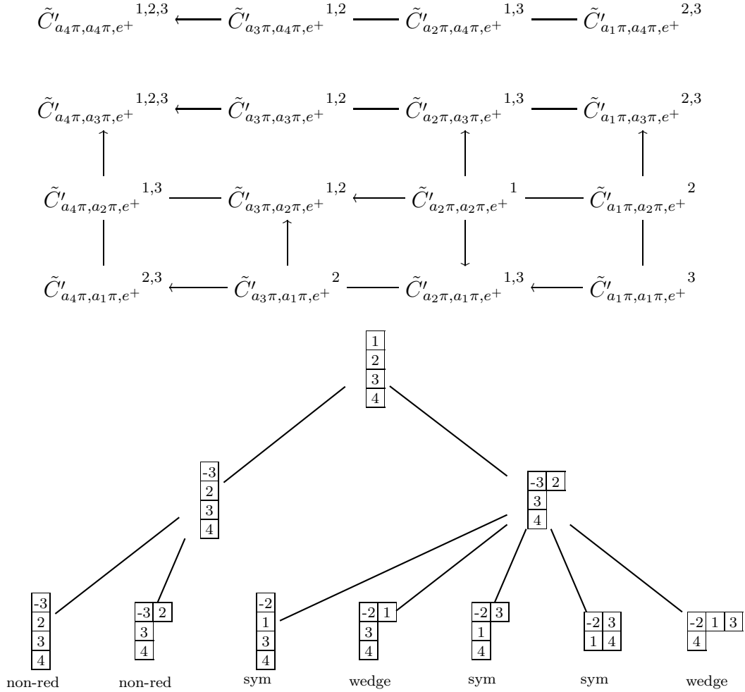
FIGURE 2. The W -graph on (\widehat{\mathcal{H}}^+ \otimes_{\mathcal{H}} (\widehat{\mathcal{H}}^+ \otimes_{\mathcal{H}} e^+)_1)_1 and the graph G of §3.4, with the labeling conventions of §4.5.
