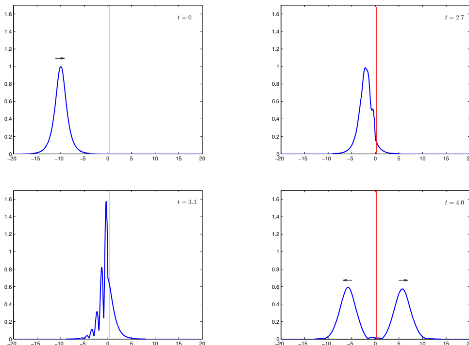
FIGURE 1. Numerical simulation of the case q = -3 , v = 3 , x_0 = -10 , at times t = 0.0, 2.7, 3.3, 4.0 . Each frame is a plot of amplitude |u| versus x .
