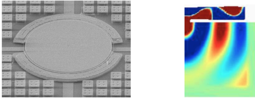
FIGURE 11. A MEMS device on the left has resonances investigated using the complex scaling/perfectly matched layer methods [BG05] – see §2.6. A numerically constructed resonant state for the elasticity operator used to model the system – see Definition 2 for a simpler case – is shown on the right.
