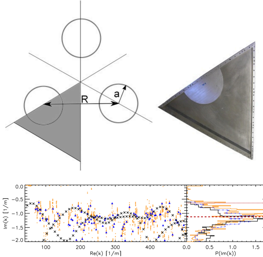
FIGURE 2. The experimental set-up for the study of the fractal Weyl law [P*12] and of the distribution of resonance widths [B*13]. On the left panel below the resonances for the aspect ratio 5.5 in the complex k -plane are shown as well as the distribution of the imaginary parts of k in the right panel. The orange clouds correspond to all resonances resulting in a good reconstruction as well as the orange histogram. Note that many orange dots might overlay each other. Blue triangles and blue dashed-dotted histogram describe the set belonging to the best reconstruction. Black crosses are the numerically calculated poles and the solid black histogram the corresponding distribution. The dotted red line in the right panel is P(1/2) , the red dashed line half of the classical decay rate P(1)/2 . Here P(s) is the topological pressure associated to the unstable Jacobian.
