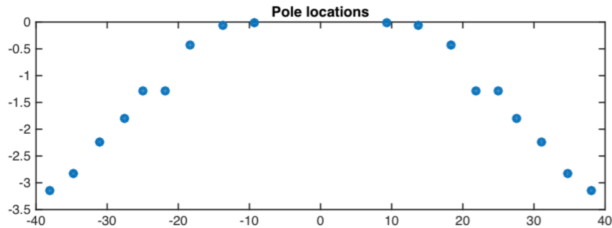
FIGURE 5. Scattering poles of the potential shown in Figure 4. They are computed very accurately using a Matlab code [BZ].
