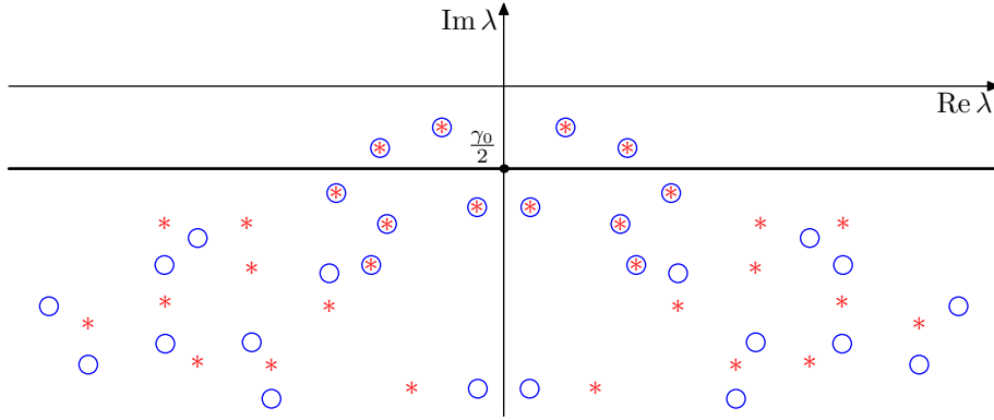
FIGURE 29. A schematic presentation of the results in Theorems 16. Pollicott–Ruelle resonances of the generator of the flow X (denoted by red asterisks) are approximated by the eigenvalues of X/i + i\varepsilon\Delta_g (denoted by blue circles) uniformly on compact sets. The asymptotic resonance free strip is uniform with respect to \varepsilon .
