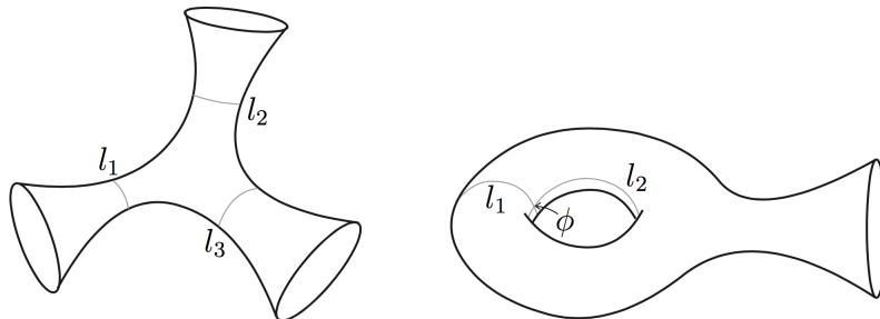
FIGURE 19. Left: surfaces X(\ell_1, \ell_2, \ell_3) with three funnels determined by lengths of the geodesic boundaries of the funnels (3.2) – see [Bo16, §16.2.1]. Right: funneled tori Y(\ell_1, \ell_2, \varphi) parametrized by the length of the two geodesics generating homotopy group of the torus and the angle between. The left example has infinity with three components; the right one with one component.
