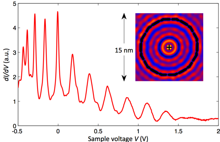
FIGURE 1. A scanning tunneling microscope (STM) spectrum is a plot of dI/dV ( I being the current) as a function of bias voltage V . According to the basic theory of STM, this reflects the sample density of states as a function of energy with respect to the Fermi energy (at V = 0 ). This spectrum shows the series of surface state electron resonances in inside a circular quantum corral on Cu(111) – see Figure 3 for a visualization of the relation between the peaks and the complex resonance poles. The bulk bands contribute to a gradually varying background in this spectrum. The setpoint was V_0 = 1\text{V} and I_0 = 10\text{nA} and the modulation voltage was V_{\text{rms}} = 4\text{mV} . Inset: a low-bias topograph of the corral studied ( 17 \times 17\text{nm}^2 , V = 10\text{mV} , I = 1\text{nA} ). The corral is made from 84 CO molecules adsorbed to Cu(111) and has an average radius of 69.28 \text{ \AA} – the data and images are from the Manoharan Lab at Stanford [M*08]. The large amplitude in the center of the top graph is a reflection of the sharp peak seen in the spectrum at V = 0 . For another quantum corral, in the shape of the Bunimovich stadium and made out of iron atoms, see Figure 14.
