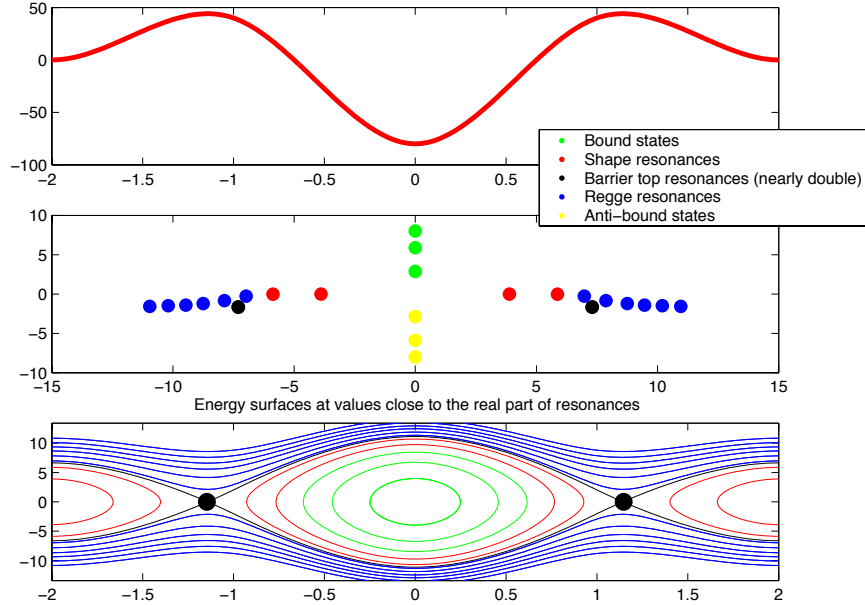
FIGURE 9. Resonances corresponding to different dynamical phenomena as poles of continuation of the resolvent \lambda \rightarrow (-h^2 \partial_x^2 + V(x) - \lambda^2)^{-1} from \text{Im } \lambda > 0 to \text{Im } \lambda \leq 0 – see §2.2. The bound states are generated by negative level sets of \xi^2 + V(x) satisfying Bohr–Sommerfeld quantization conditions. Bounded positive level sets of \xi^2 + V(x) can also satisfy the quantization conditions but they cannot produce bound state – tunnelling to the unbounded components of these level sets is responsible for resonances with exponentially small ( \sim e^{-S/h} ) imaginary parts/width. The unstable trapped points corresponding to maxima of the potential produce resonances which are at distance h of the real axis.
