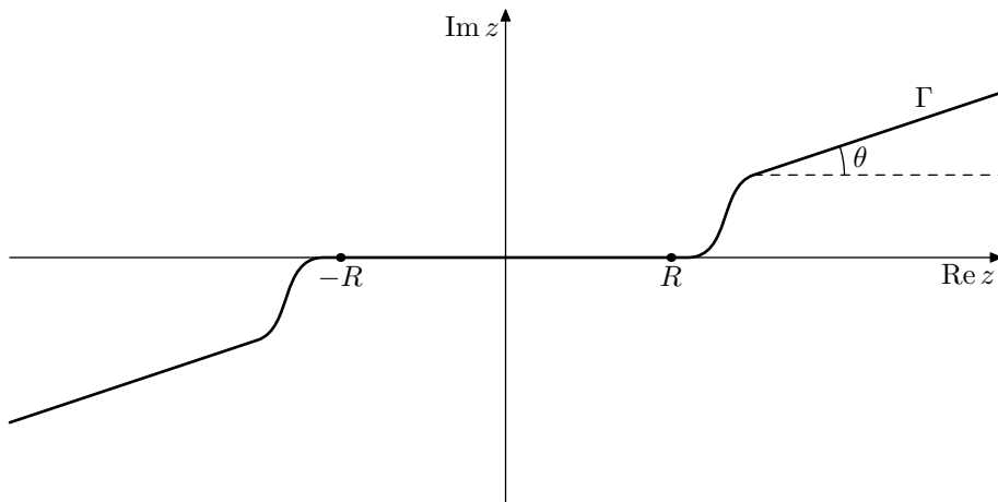
FIGURE 17. Curve \Gamma used in complex scaling. The curve is given by x \mapsto x + ig(x) for a C^\infty function g satisfying g(x) = 0 for -R \leq x \leq R and g(x) = x \tan \theta for |x| sufficiently large, where \theta is a given constant.
