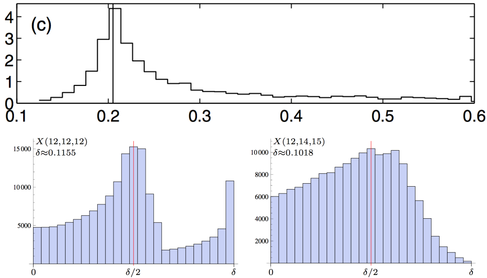
FIGURE 26. Top: histogram of imaginary parts of resonances of a three discs configuration (see Figure 2) with real parts with |\operatorname{Re} \lambda| \leq 2 \times 10^3 computed using a semiclassical zeta function [LSZ03]. The imaginary parts concentrate at \frac{1}{2}\mathcal{P}_1(1) , that is at one half of the classical escape rate. (We should remark here that the method of calculation based on the zeta function, although widely accepted in the physics literature, does not have a rigorous justification and may well be inaccurate. However, the phenomenon of concentration at \frac{1}{2}\mathcal{P}_1(1) has been verified experimentally – see [B*13] and Figure 10). Bottom: histograms from Borthwick [Bo14] showing the distribution of imaginary parts (the x axis is \operatorname{Im} \lambda + \frac{1}{2} ) for hyperbolic surfaces X(\ell_1, \ell_2, \ell_3) (see Figure 19) with |\operatorname{Re} \lambda| \leq 2 \times 10^4 . The concentration at \operatorname{Im} \lambda = \frac{1}{2}(\delta - 1) is clearly visible. Recalling (3.27) and (3.31) that is the same as in the top figure.
