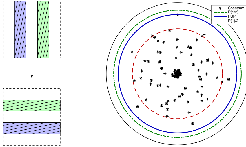
FIGURE 23. Left: a schematic representation of an open baker map (a piecewise smooth symplectic relation) \kappa_{M,\mathcal{A}}: \mathbb{R}^2/\mathbb{Z}^2 \ni (y, \eta) \mapsto (My-a, (\eta+a)/M) , (y, \eta) \in (a/M, (a+1)/M) , a \in \mathcal{A} \subset \{0, \dots, M-1\} , here with M = 5 , \mathcal{A} = \{1, 3\} . A quantization, B_{5N} , of this open map (relation) is given in (3.38). Right: resonances of B_{5N} with N = 5^4 . Different theoretical gaps are also shown: for this quantum map the fractal uncertainty principle (FUP) of [DJ16],[DZ15] does produce an optimal gap.
