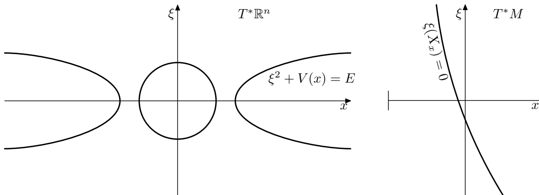
FIGURE 27. Scattering in \mathbb{R}^n and Anosov flows on a compact manifold M : the classical Hamiltonians in phase space (now a “double phase space” in case of Anosov flow, T^*M ) are p(x, \xi) = |\xi|^2 + V(x) , (x, \xi) \in T^*\mathbb{R}^n and p(x, \xi) = \xi(X_x) , (x, \xi) \in T^*M (where X generates the Anosov flow). In both cases, the energy surfaces p = E are non-compact : in scattering x \rightarrow \infty , in the Anosov case, \xi \rightarrow \infty . Figure 28 below should be compared to [Me94, Figure 2]: it is not surprising that Melrose’s “radial estimates” play a role in the analysis of both cases. For flows the situation is simpler since the flow is linear in the \xi variables (see (4.6)) and there is no additional infinity (in the scattering case there is also the \xi infinity). When M is non-compact the situation becomes more complicated as both infinities play a role: see [DG14, Figure 2].
