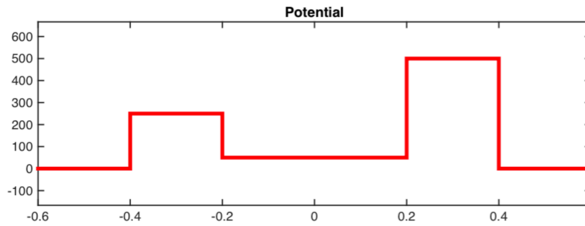
FIGURE 4. A simple one dimensional potential with resonances shown in Figure 5. Same potential is used to see propagation, trapping and tunneling of a wave in Figure 6.
