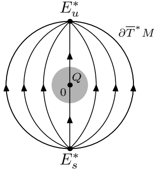
FIGURE 28. A schematic representation of the flow on the compactification of T^*M , \bar{T}^*M – by compactification we mean replacing each fiber T_x^*M by a ball \bar{T}_x^*M with the boundary corresponding to the sphere at infinity. At zero energy, p^{-1}(0) = \{(x, \xi) : \xi(X_x) = 0\} the trapped set of the flow is given by the zero section and the operator X/i - iQ(x, hD)/h - \lambda is invertible on spaces H_{rG} (with uniform bounds once the norms are semiclassical modified by changing G(x, D) to G(x, hD) ) for Q \geq 0 microlocalized to the shaded region and elliptic in a neighbourhood of the trapped set and \text{Im } \lambda > -r/C_0 . Since Q(x, hD) is a compact operator that, and estimates on the adjoint on dual spaces, shows the Fredholm property of X/i - \lambda .
