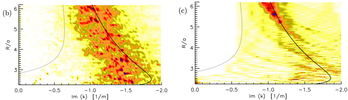
FIGURE 10. Distribution of resonance width (decay rates) for a three disc scatterer [B*13] in a symmetry reduced microwave model shown in Figure 2: the plots show the density of values of resonance width, \text{Im } k , for a range of rest frequencies ( 40\text{m}^{-1} \leq \text{Re } k \leq 500\text{m}^{-1} ) against the aspect ratio of a three disc system (see Figure 2). The experimental data (left) and numerical data (right) are compared. The dotted line shows the topological pressure at \frac{1}{2} and the solid line \frac{1}{2} of the classical decay rate as functions of the aspect ratio. The former predicts the resonance free region and the latter, the concentration of decay rates.
