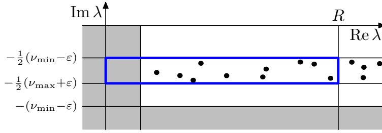
FIGURE 22. A schematic presentation of the results of [Dy15a] for an operator -\Delta_g with an r -normally hyperbolic trapped set. Here R = 1/h and we use the resolvent (-\Delta_g - \lambda^2)^{-1} . The resonance free strip is the same as in Theorem 10 and the resonances in the strip \text{Im } \lambda > -\frac{1}{2}(\nu_{\max} + \varepsilon) satisfy a Weyl law: |\{\lambda : \text{Im } \lambda > -\frac{1}{2}(\nu_{\max} + \varepsilon), 0 < \text{Re } \lambda < R\}| \sim R^{n-1} \text{vol}(K_{[0,1]}) / (2\pi)^{n-1} – see [Dy15a, Theorem 3].
