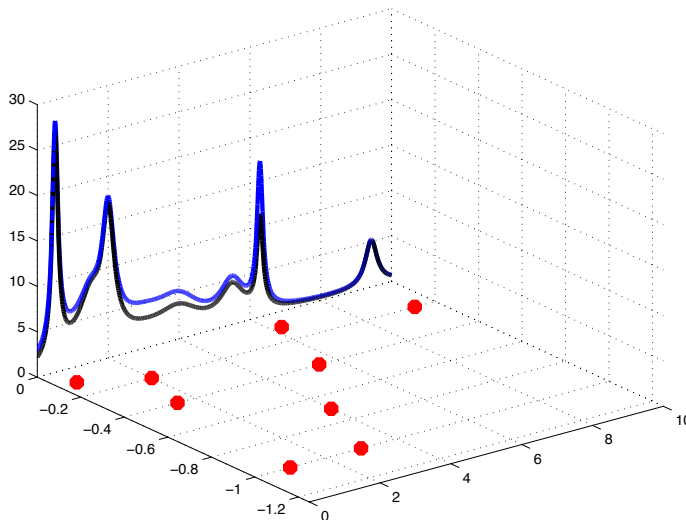
FIGURE 3. If U(t) is a propagator and f, g are states then the correlation (the evolution of f measured by g ) is given by \rho_{f,g}(t) = \langle U(t)f, g \rangle . For instance the evolution could come from a flow \varphi_t : M \rightarrow M on a compact manifold, U(t)f(x) = f(\varphi_{-t}(x)) . The power spectrum of correlations is given by \widehat{\rho}_{f,g}(\lambda) := \int_0^\infty \rho_{f,g}(t)e^{i\lambda t} dt . Resonances are the poles of \widehat{\rho}_{f,g}(\lambda) and are independent of f and g . The figure shows a schematic correspondence between the power spectrum for different states and these poles: the real part corresponds to the location of a peak in the power spectrum and the imaginary to its width; the x axis is the real part (frequency \lambda ), y axis the imaginary (rate of decay), z axis |\widehat{\rho}_{f,g}(\lambda)| . Unlike the power spectrum which depends on f and g , the poles depend only on the system.
