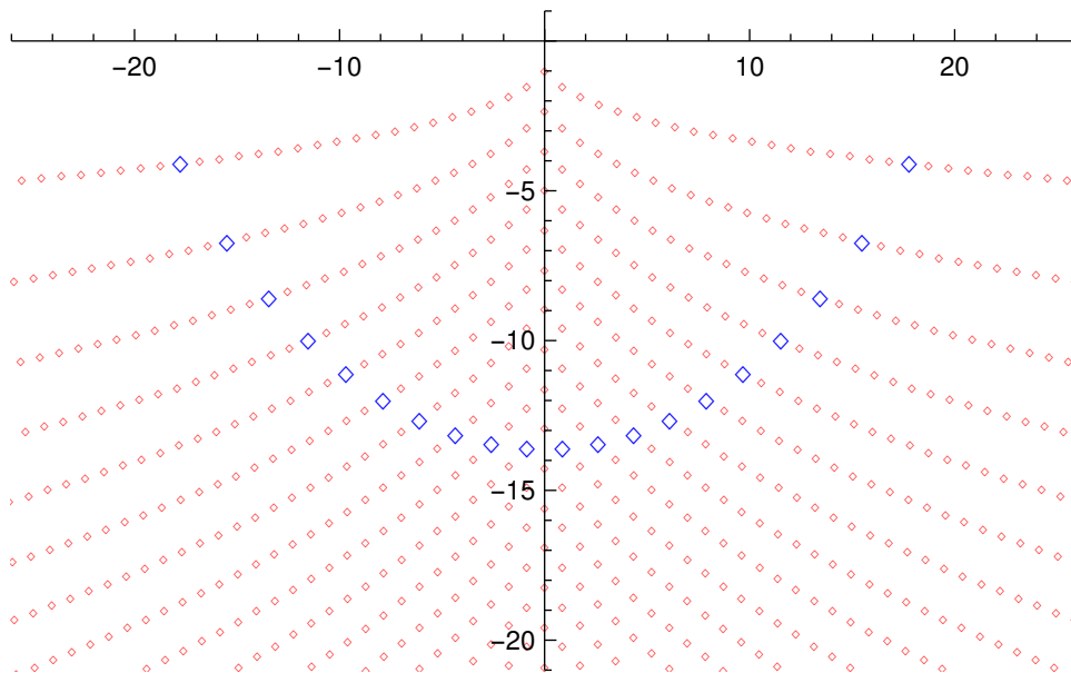
FIGURE 8. Resonances for the sphere in three dimensions. For each spherical momentum \ell they are given by solutions of H_{\ell+\frac{1}{2}}^{(2)}(\lambda) = 0 where H_{\nu}^{(2)} is the Hankel function of the second kind and order \nu . Each zero appears as a resonance of multiplicity 2\ell + 1 : the resonances with \ell = 20 are highlighted.
