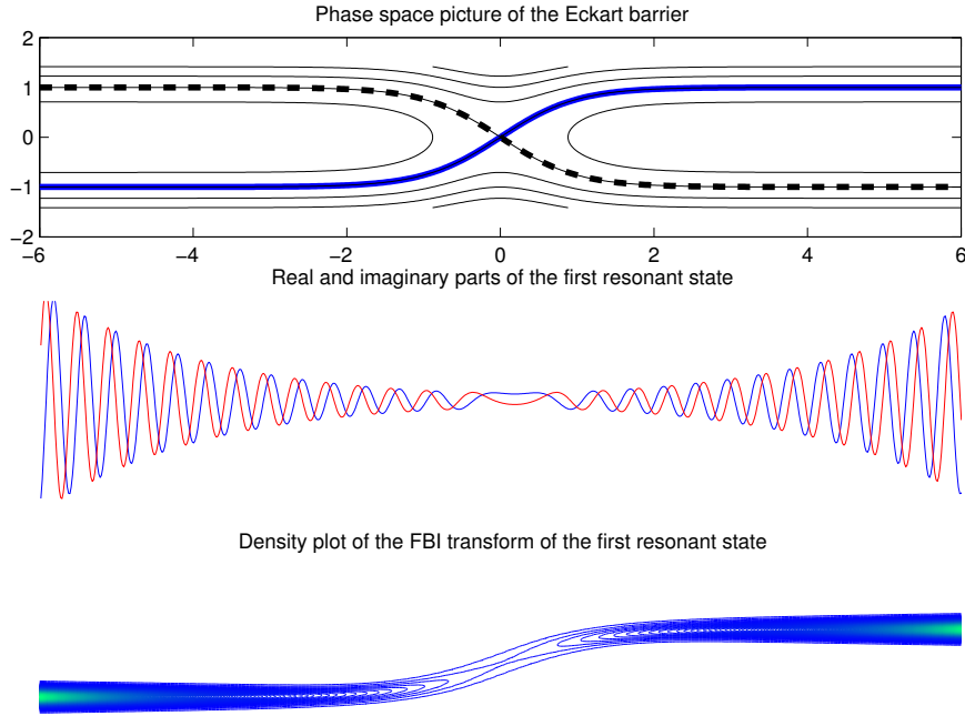
FIGURE 25. The top figure shows the phase portrait for the Hamiltonian p(x, \xi) = \xi^2 + \cosh^{-2}(x) , with \Gamma_1^\pm highlighted. The middle plot shows the resonant state corresponding to the resonance closest to the real axis at h = 1/16 (compare this to the resonances in Figure 9 generated by the local maxima), and the bottom plot shows the squared modulus of its FBI transform (which describes a wave function in phase space [Zw12, Chapter 13]). The resonance states were computed by D. Bindel [BZ] and the FBI transform was provided by L. Demanet. We see that the mass of the FBI transform is concentrated on \Gamma_1^+ , with the exponential growth in the outgoing direction. See also https://www.youtube.com/watch?v=R7eUpEVpckk&feature=youtu.be&list=PL32oQ9j10WcORi1NwnY6BtDawepnBnQyx
