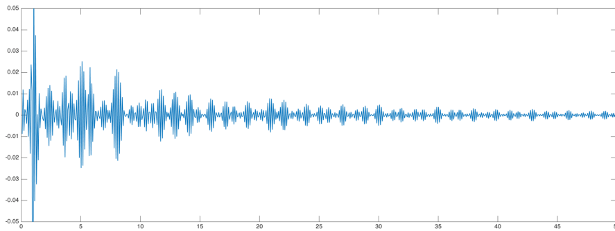
FIGURE 7. The plot of u(0, t) showing oscillations and decay of the solution from Figure 6 in the interaction region. The principal decay rate of the wave is determined by the resonance(s) closest to the real axis. For that we need to justify the expansion (1.2) – see Theorem 5.
