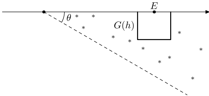
FIGURE 20. The meromorphic continuation (3.21): The resonances of P are identified with the eigenvalues the scaled operator P_\theta constructed by a higher dimensional version of the method presented in §2.6. Resonances are studied near a fixed energy level in a neighbourhood of size depending on h .
