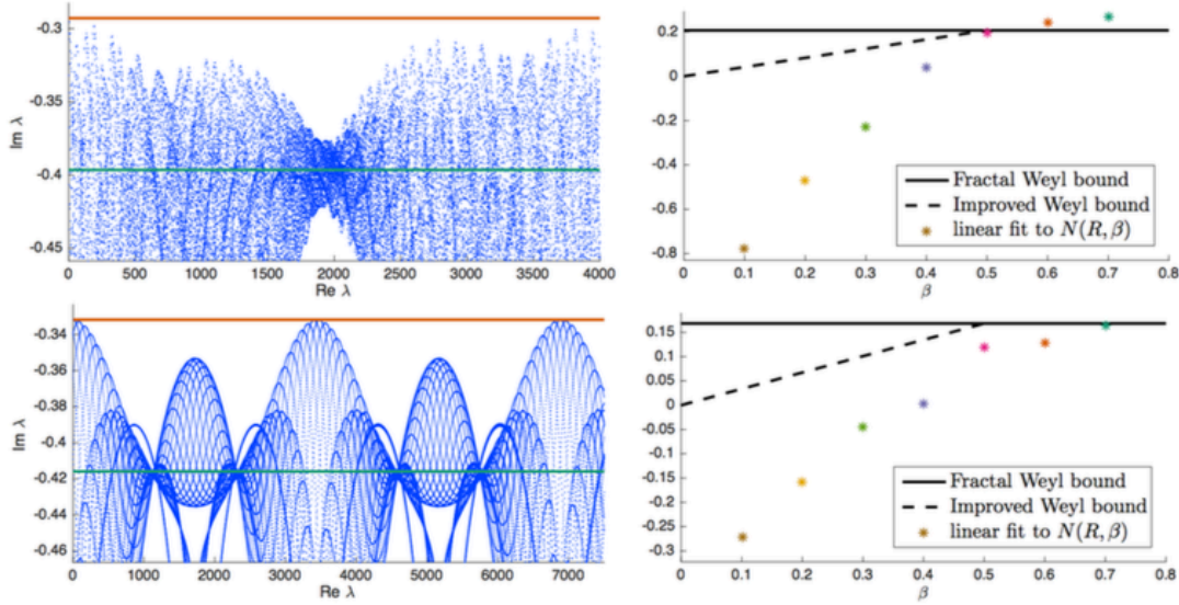
FIGURE 21. Left: resonances for X(6, 7, 7) and Y(7, 7, \pi/2) from [Dy16b, Appendix] (see Figure 19 for the definition and picture of these surfaces; here we show the poles of the continuation of (-\Delta_g - \lambda^2 - \frac{1}{4})^{-1} ). The top line is the pressure gap (3.33) with P(\frac{1}{2}) = \frac{1}{2} - \delta . The lower line is given by half of the classical decay rate, P(1)/2 = (1 - \delta)/2 where \delta is the dimension of the limit sets for the two surfaces – see (3.31). Right: numerical illustration of Theorems 13 and 14 with the standard [GLZ04],[DD13] and improved [Dy16b] fractal Weyl laws – see §3.4 – for the corresponding surfaces; here N(R, \beta) is the number of resonances in |\operatorname{Re} \lambda| \leq R , \operatorname{Im} \lambda > \frac{1}{2} + (\beta - 1)\delta . The “chain patterns” visible on the left (which are even more pronounced for more symmetric systems such as X(\ell, \ell, \ell) – see [BW16]) have been recently investigated by Weich [We15].
