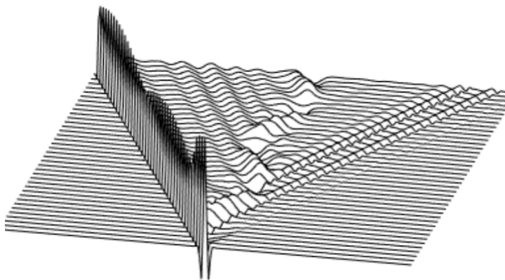
FIGURE 6. A solution of the wave equation \partial_t^2 u - \partial_x^2 u + Vu = 0 where V is shown in Figure 4. The initial data is localized near 0 and the time variable t points away from the viewer.
