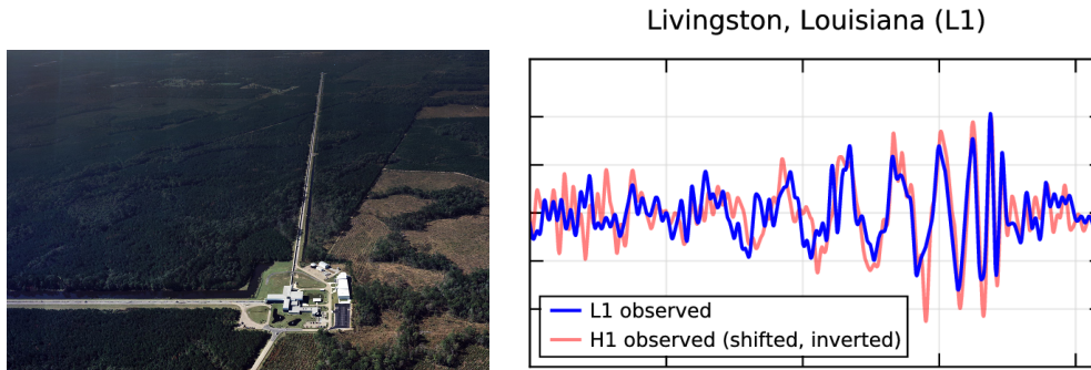
FIGURE 12. Left: an aerial view of the LIGO laboratory in Livingston, Louisiana, US. Right: the gravitational wave signal observed on September 14, 2015 simultaneously by LIGO Livingston (blue) and LIGO Hanford (red); see [A*16]. Quasi-normal modes, as scattering resonances are called in the context of gravitational waves, are supposed to appear in the “ring-down phase” but have not been observed yet. The picture is obtained from the LIGO Open Science Center, https://losc.ligo.org , a service of LIGO Laboratory and the LIGO Scientific Collaboration. LIGO is funded by the U.S. National Science Foundation.
