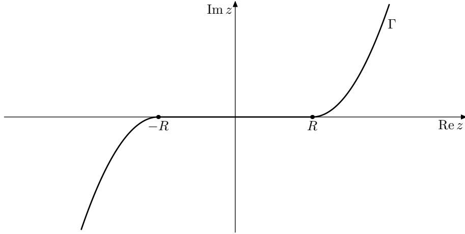
FIGURE 18. Curve \Gamma used in PML computations – see [BG05] and references given there. A typical curve is given by a function \mathbb{R} \ni x \mapsto x + ig(x) where g(x) = -|x+R|^\alpha for x < -R , g(x) = 0 for -R \leq x \leq R , and g(x) = (x-L)^\alpha for x > R , where \alpha > 1 .
