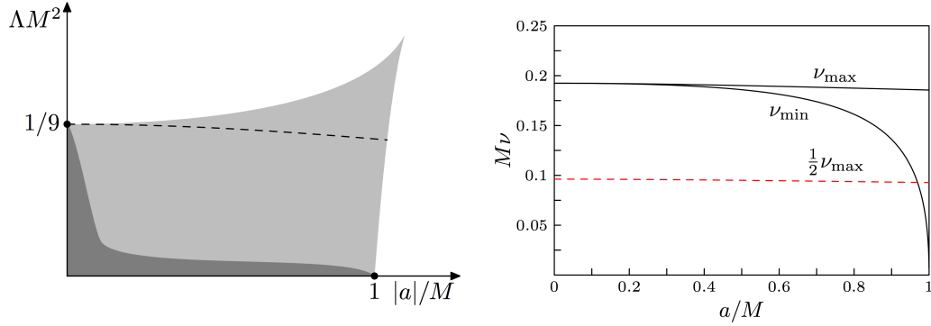
FIGURE 24. Left: numerically computed admissible range of parameters for the subextremal Kerr–de Sitter black hole (light shaded) and the range to which the resonance expansions of [Dy15b] apply. QNM are defined and discrete for parameters below the dashed line, (1 - \Lambda a^2/3)^3 = 9\Lambda M^2 , see [Dy15b, §3.2]. Right: The dependence of \nu_{\max} and \nu_{\min} on the parameters M and a in the case of \Lambda = 0 . The dashed line indicates the range of validity of the pinching condition needed for the Weyl law [Dy15a] recalled in Figure 22.
