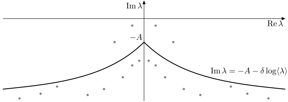
FIGURE 16. The contour used to obtain the resonance expansion.
