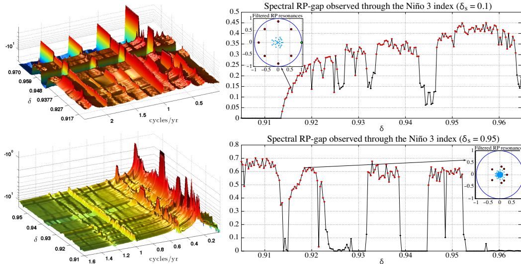
FIGURE 13. Left: Parameter (denoted by \delta ) dependence of power spectra of El Niño models considered in [C*14]. Right: the dependence of the spectral gap on the same parameter \delta ; here the resonance of maps obtained by using Markov partitions are presented and they lie inside of the unit disk. The resonance for flows are obtained by taking logarithms which is similar to the case of resonances of quantum maps – see Figure 23.
