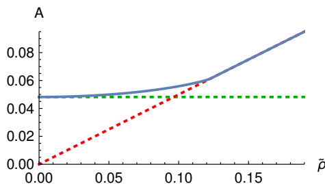
FIGURE 5. Estimates for the resonance width \alpha = A/\rho . Blue : graph of A(\tilde{\rho}) . Green : A \equiv \mu , corresponding to the Euclidean estimate (5.9). Red : A = \frac{1}{2}\tilde{\rho} , corresponding to the unconditional bound (1.5).
