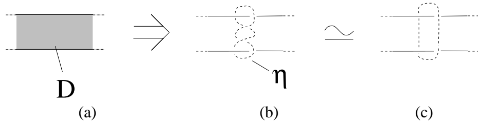
F 4.1. Infection by a knot.
