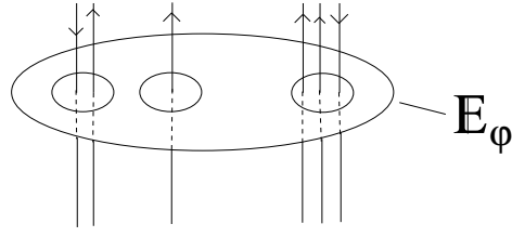
F 1.3. Properly embedded multi-disk.
