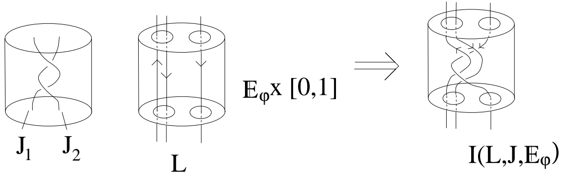
F 1.4. Multi-infection of L by J .
