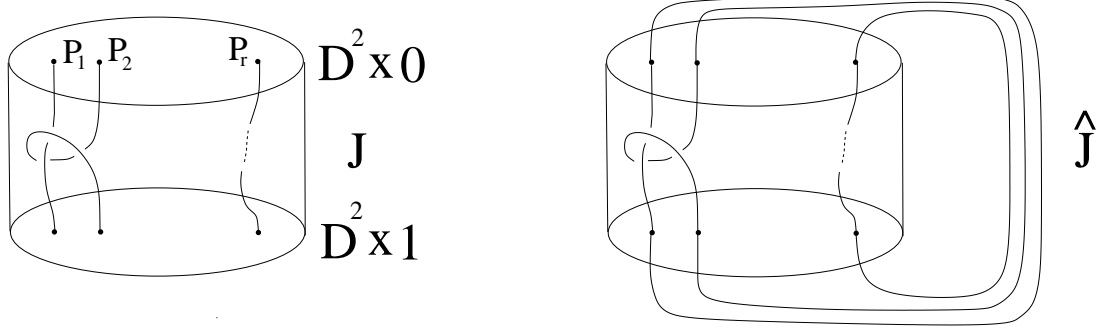
F 2.2. String link and its closure.
