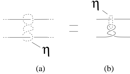
F 4.2. Isotopy of K \cup \eta .
