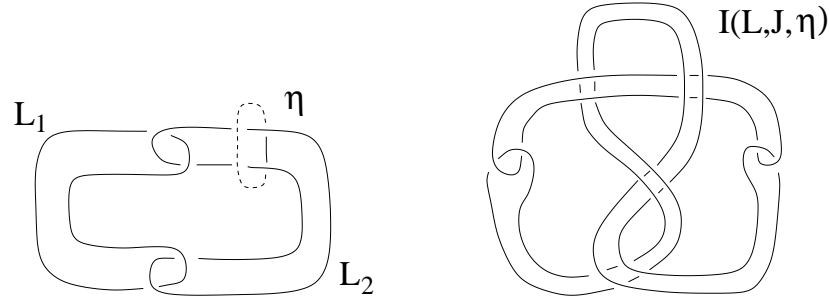
F 4.4. Satellite construction with \hat{J} the figure 8 knot, and L the trivial 2–component link.
