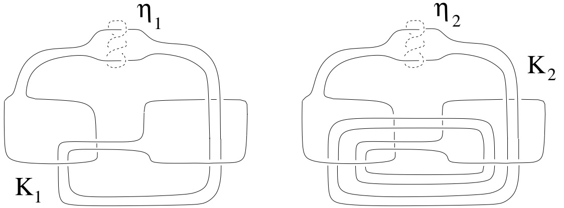
F 4.3. The knots K_1 and K_2 with curves \eta_1 and \eta_2 .
