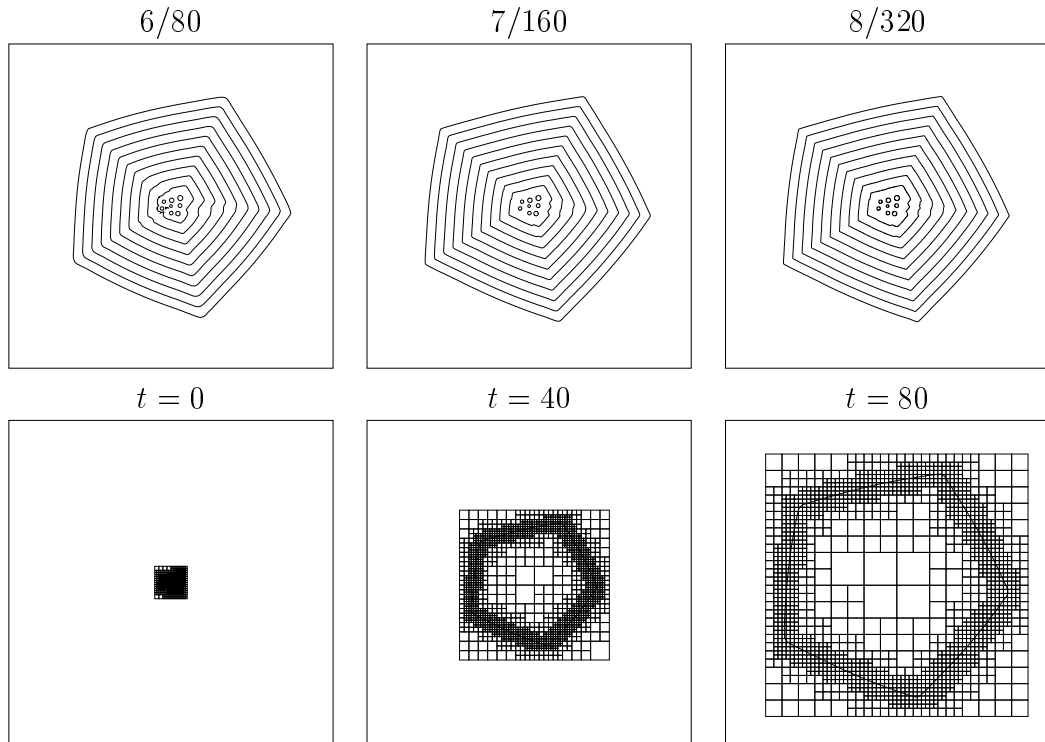
Figure 16: Bubbles merging into the asymptotic Wulff shape.
