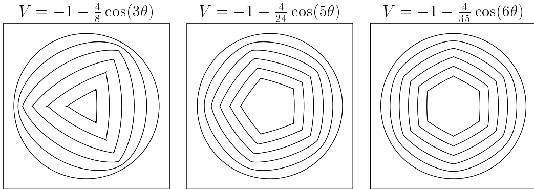
Figure 14: Radius 3.5 circles shrinking into the asymptotic Wulff shapes: 6/40 vs 7/80 runs for 0 \leq t \leq 2 on [-4, 4]^2 .
