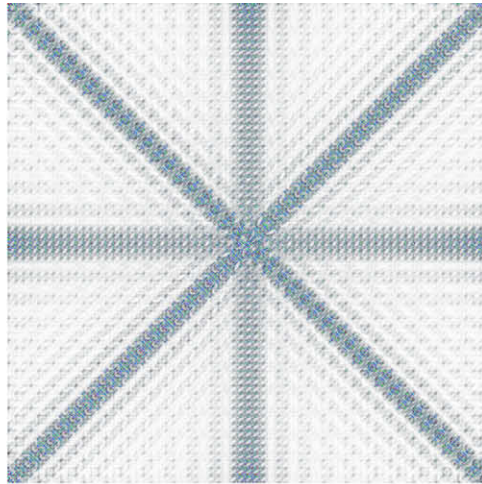
(b) 5 iterations
