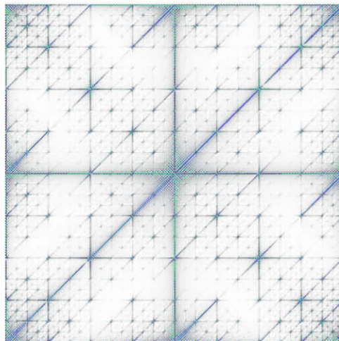
(f) 15 iterations
