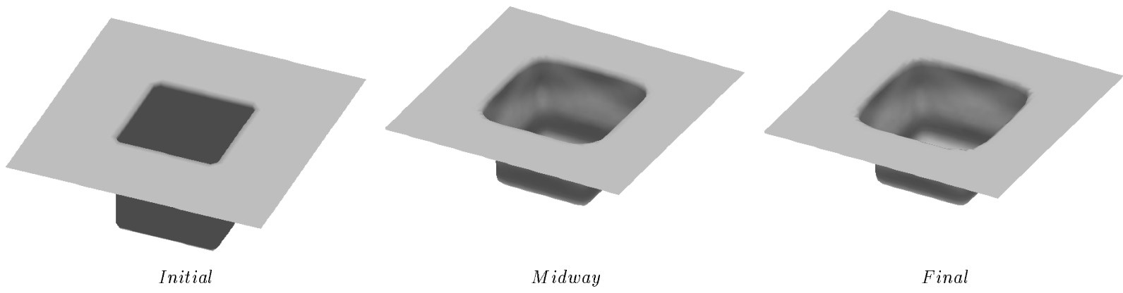
Figure 11: Source Etching into Hole
