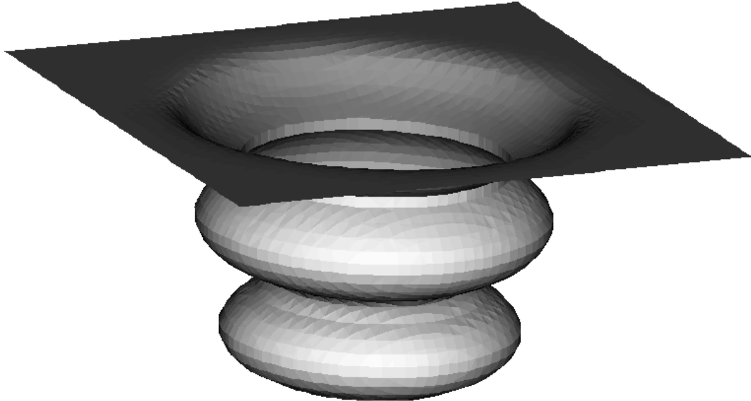
Figure 12: Lithography: 2nd Order: Grid Size=50x50x47
