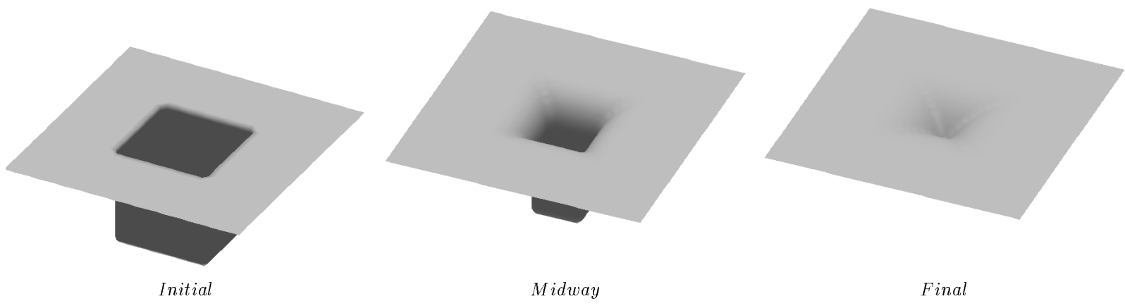
Figure 6: Isotropic Deposition into Hole
