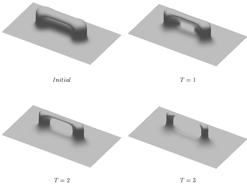
Figure 15: Isotropic Etching of Bridge
