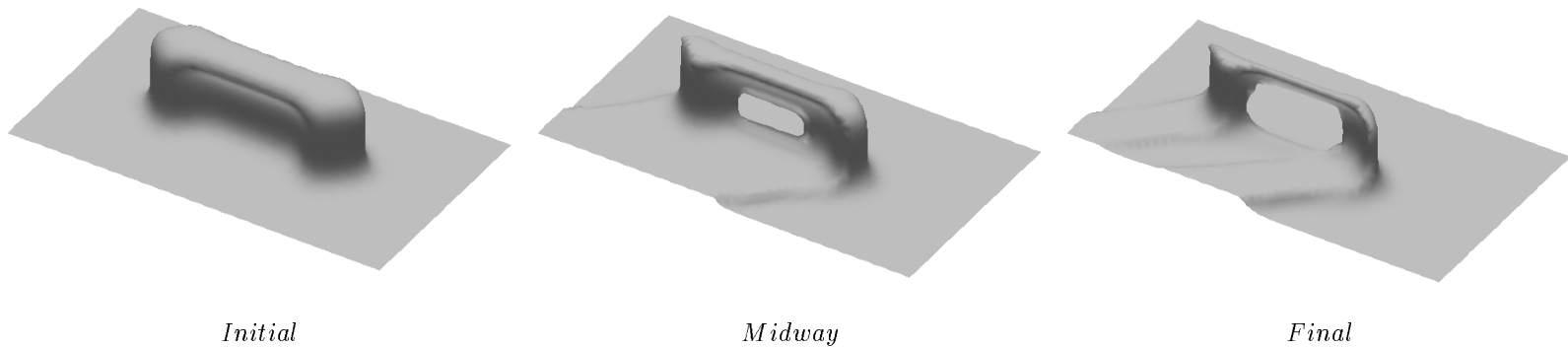
Figure 16: UniDirectional Etching of Bridge
