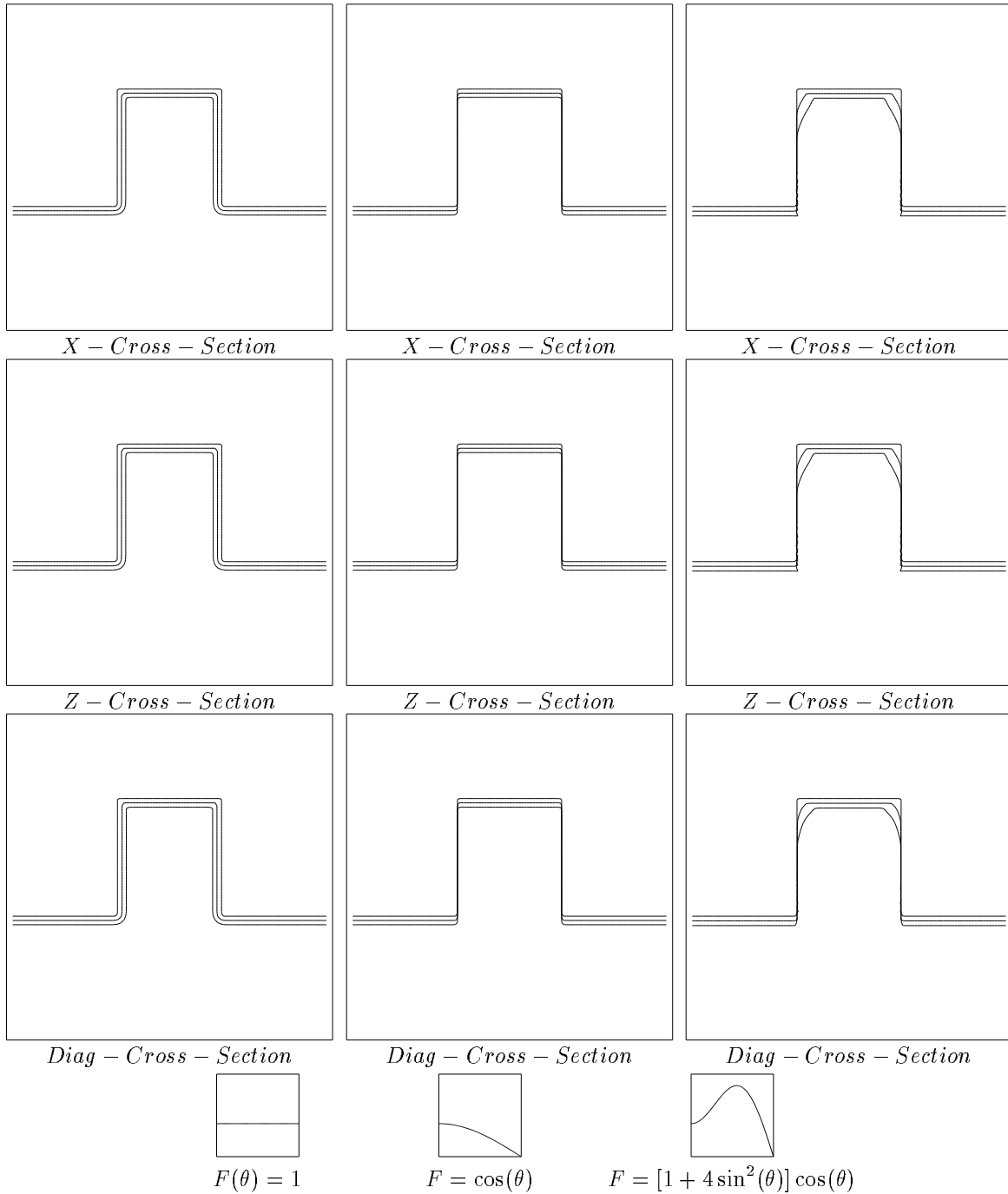
Figure 18: Three Dimensions: Effects of Different Yield Functions
