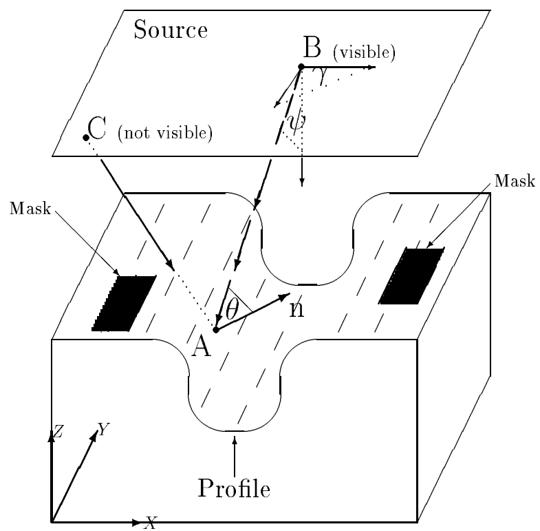
Figure 5: Variables and Setup
