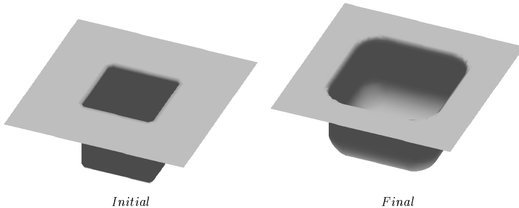
Figure 9: Isotropic Etching into Hole
